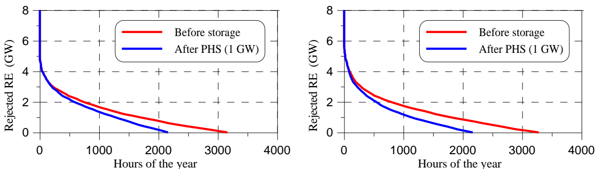
Figure 3.5. Duration curves of RES rejected production for 40% RES share (2020-MEAP), and cases A (left), and B (right).
