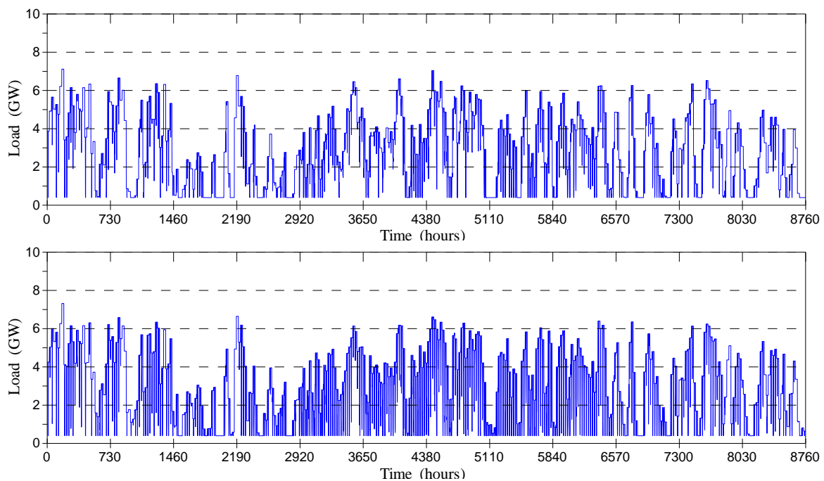
Figure 3.12. CPL curve after full PHEs exploitation, for 80% RES share – case A (upper), case C (lower).
