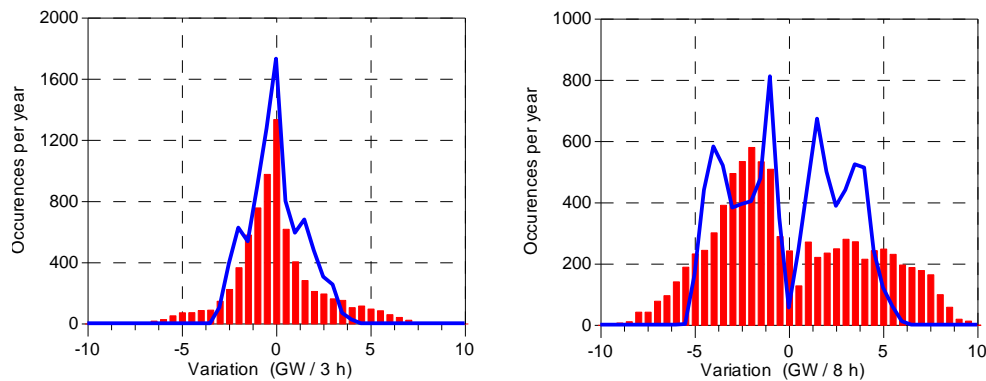
Figure 2.8. Variation of the system Load (lines) and Controllable Plants Load (bars) for the 80% scenario – Case C.
