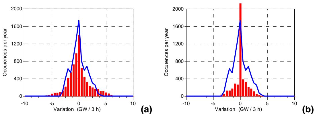
Figure 6. Variation of System Load (lines) and of Controllable Plants Load (bars) for the 80% scenario – case A. a) Without PHES, and b) after full PHES exploitation).
