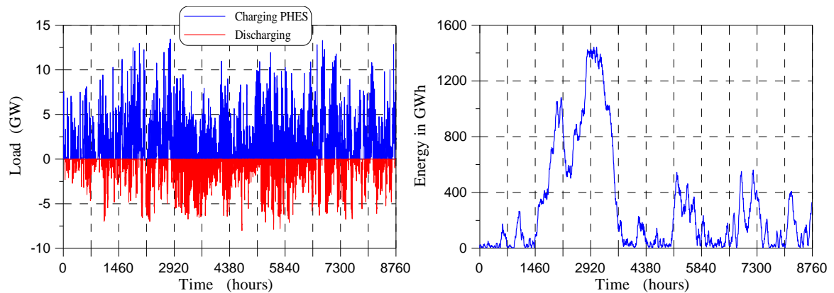
Figure 3.26. Power and charging level for unlimited storage power and capacity and higher system technical minimum – case A.
