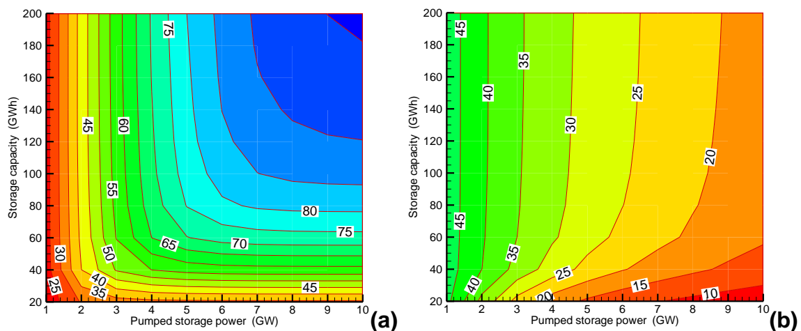
Figure 9. Hill charts of RES energy storage efficiency and CF of pumping units, for 80% scenario – case C.
