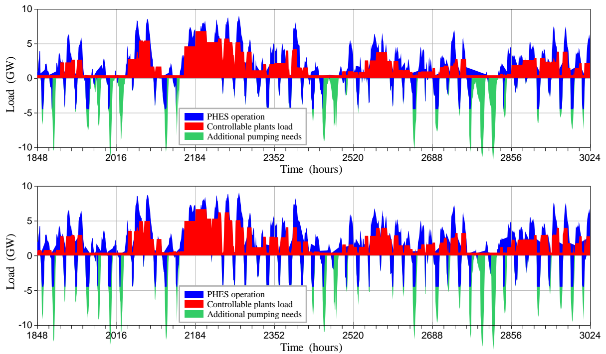
Figure 3.13. PHEs and Controllable plants load variation for 80% scenario – case A (upper), case C (lower).
