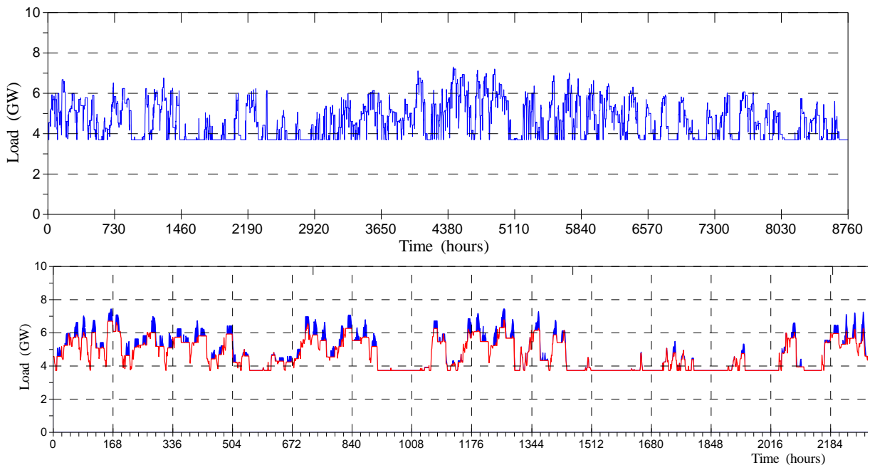
Figure 3.3. Controllable Plants Load after full PHES exploitation (upper) and detailed view of peak shaving effect (lower) – case A.
