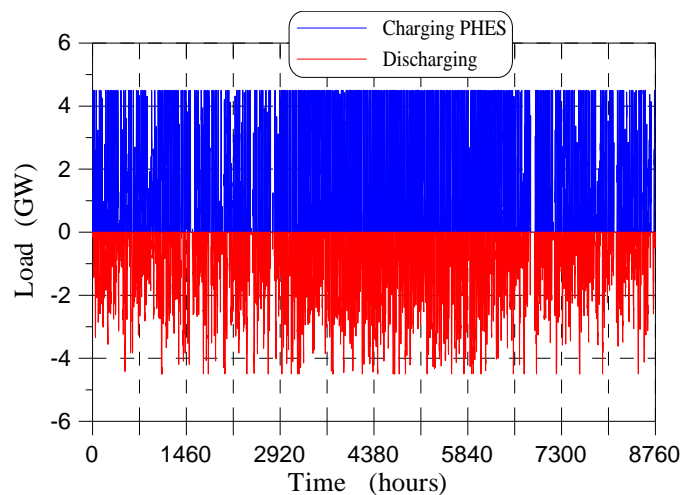
Figure 3.17. Power level after full exploitation of the PHEs system – cases A
