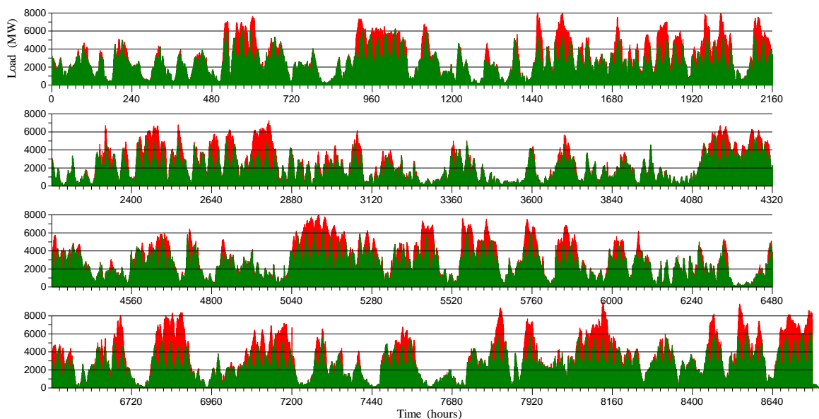
Figure A4. Time history of wind production in the year 2050 and MEAP scenario: Green=absorbed in the grid; Red=rejected, for storage.
