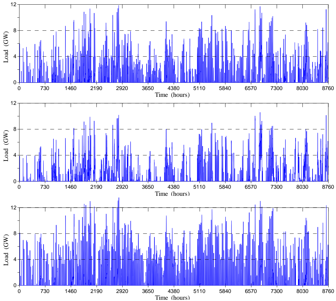
Figure 2.5. Rejected energy from intermittent RES for 80% scenario, and cases A, B and C (from top to bottom).
