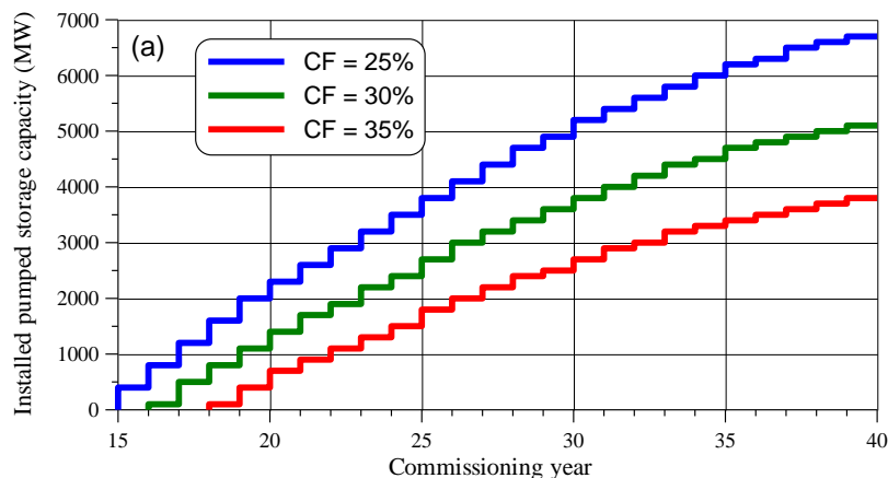
Figure 10. Optimum sizing of PHES development up to 2040 for the MEAP scenario.
