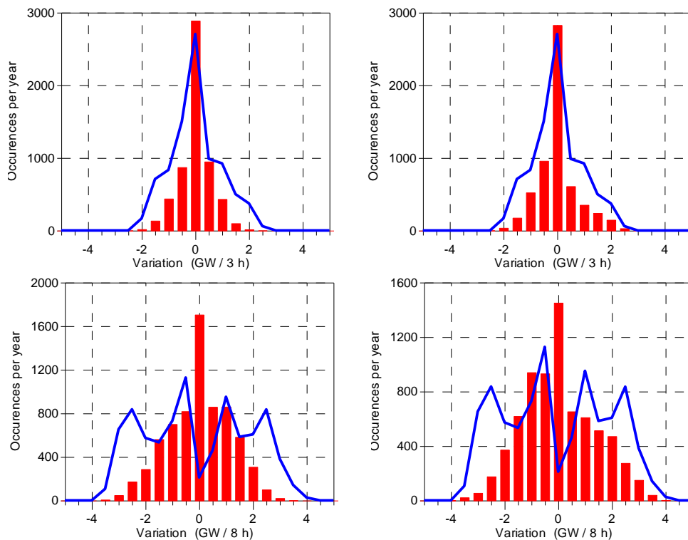
Figure 3.9. Total load variation (cont. lines) and Controllable Plants Load with the PHES (bars) for the 40% scenario: Case A (left), and case B (right).
