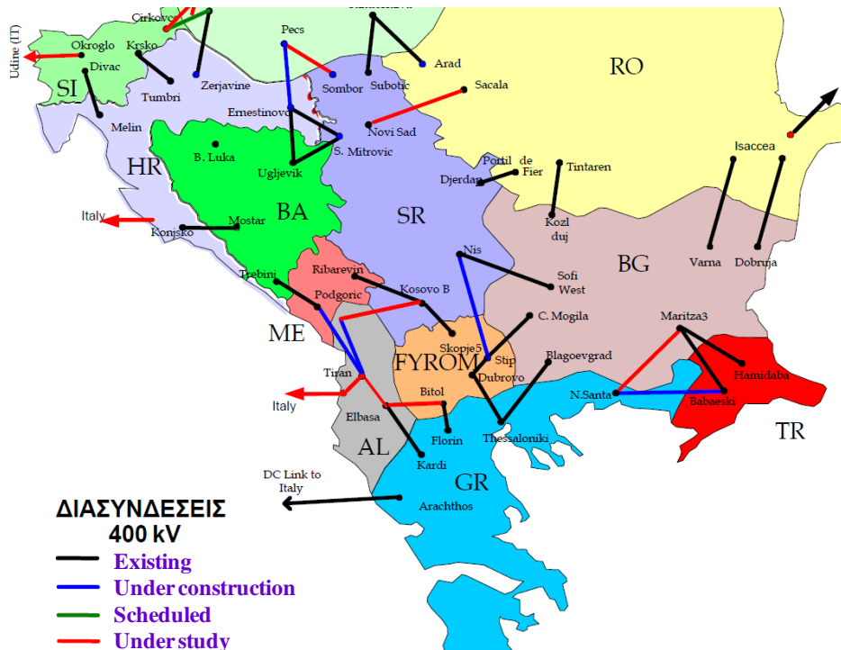
Figure 1.3. Topology of existing and future connections in the ENTSO-E system
