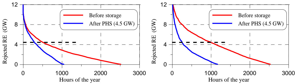
Figure 3.14. Duration curves of RES rejected production for 80% RES share and cases B (left), and C (right).
