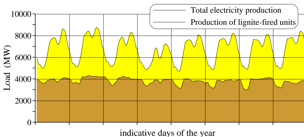
Figure A1. Indicative electricity generation history curves in the Greek system.
