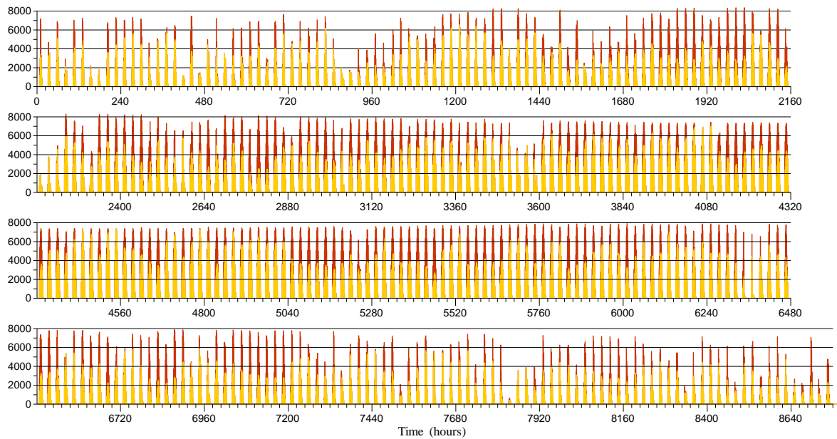
Figure A5. Time history of PV production in the year 2050 and MEAP scenario: Yellow=absorbed in the grid; Red=rejected, for storage.
