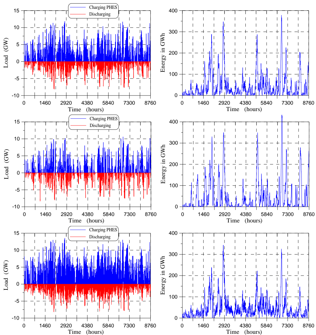
Figure 3.25. Power and charging level for storage system with unlimited power and capacity, for 80% share – cases A, B and C (top to bottom).
