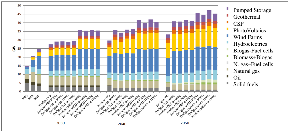
Figure 1.10. Installed capacity of electricity production technologies for various development scenarios [5].
