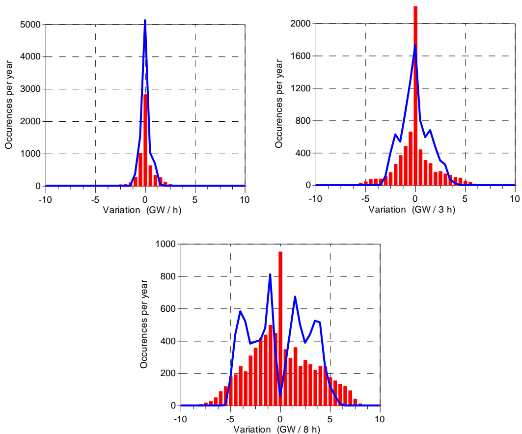
Figure 3.19. Total load variation (cont. lines) and Controllable Plants Load variation with the PHES (bars) for rejected RES production and 80% scenario – case A.
