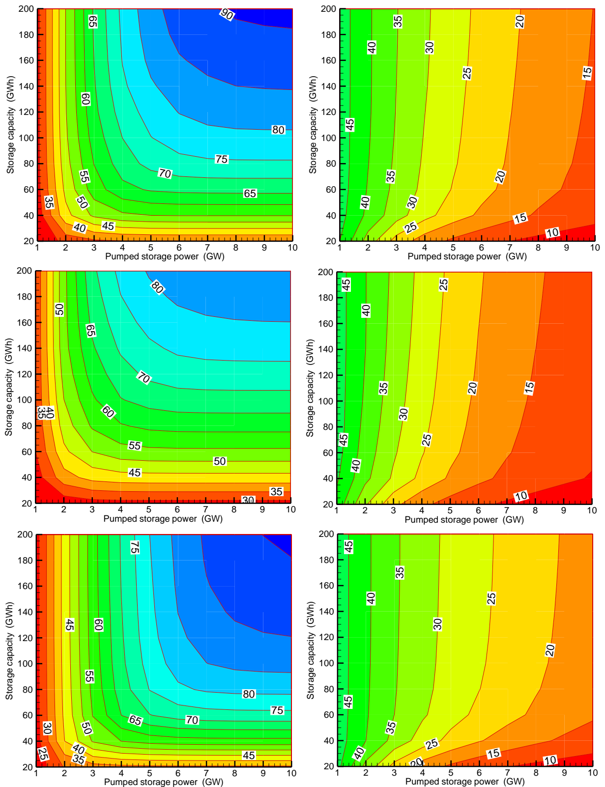
Figure 3.27. Effect of installed pumped storage power and capacity on the RES rejections exploitation degree (left), and on the capacity factor of pumping units (right). 80% RES share scenario – cases A, B, C (top to bottom).
