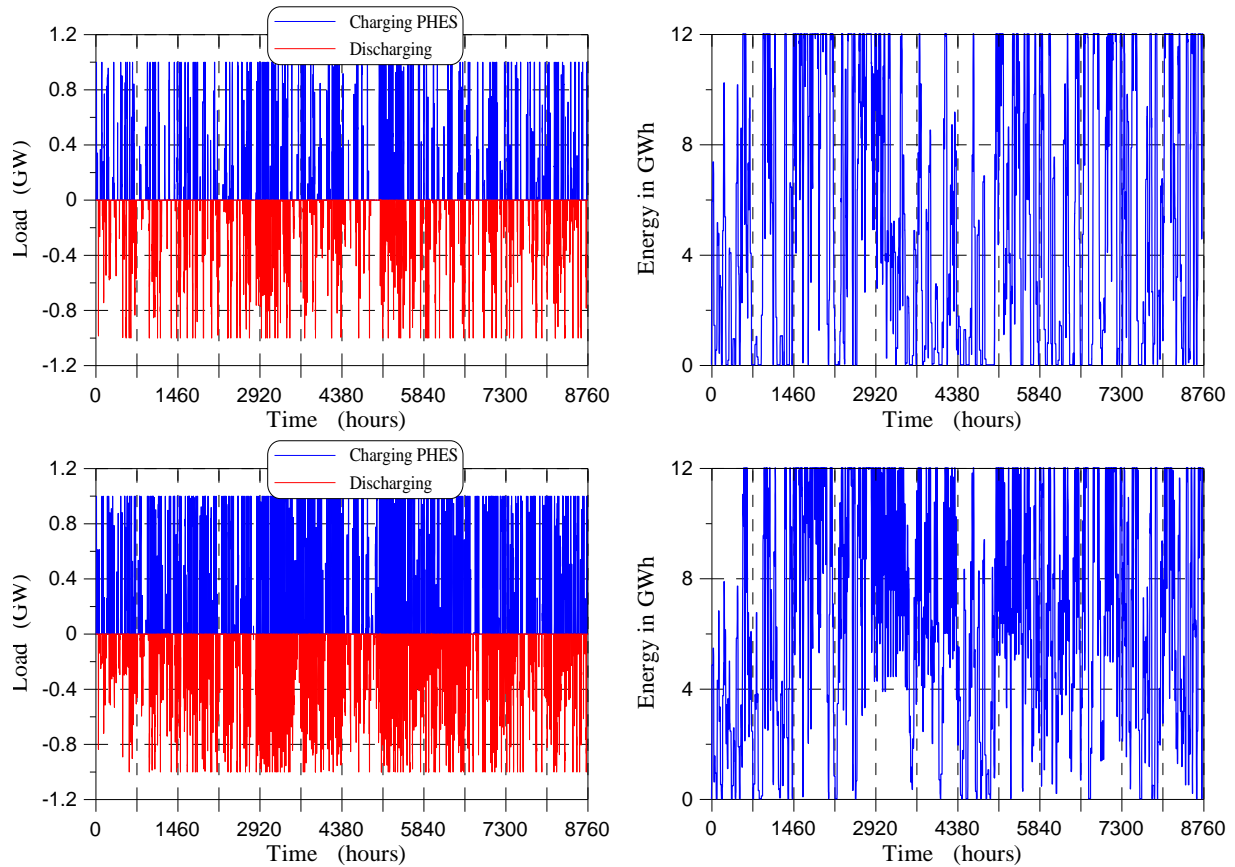
Figure 3.7. Power and charging level of the PHEs system only for RES storage, for 40% share – cases A (upper), and B (lower).
