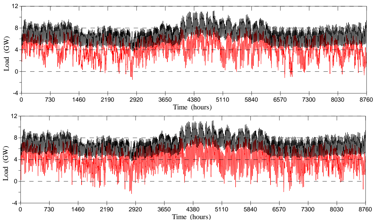
Figure 2.1. Load (black) and residual load (red) for the 40% RES share (2020-MEAP scenario), and cases A (upper) and B (lower).
