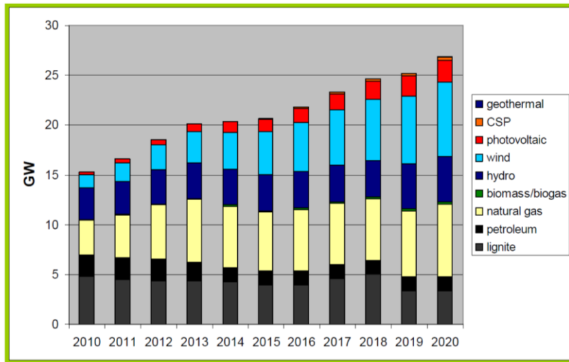
Figure 1.7. Estimated installed power for electricity production (National RES action plan 2010).
