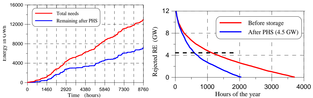
Figure 3.18. Results for higher RES penetration limit – case A. Accumulated RES rejections during one year (left), and duration curves of rejected production (right).
