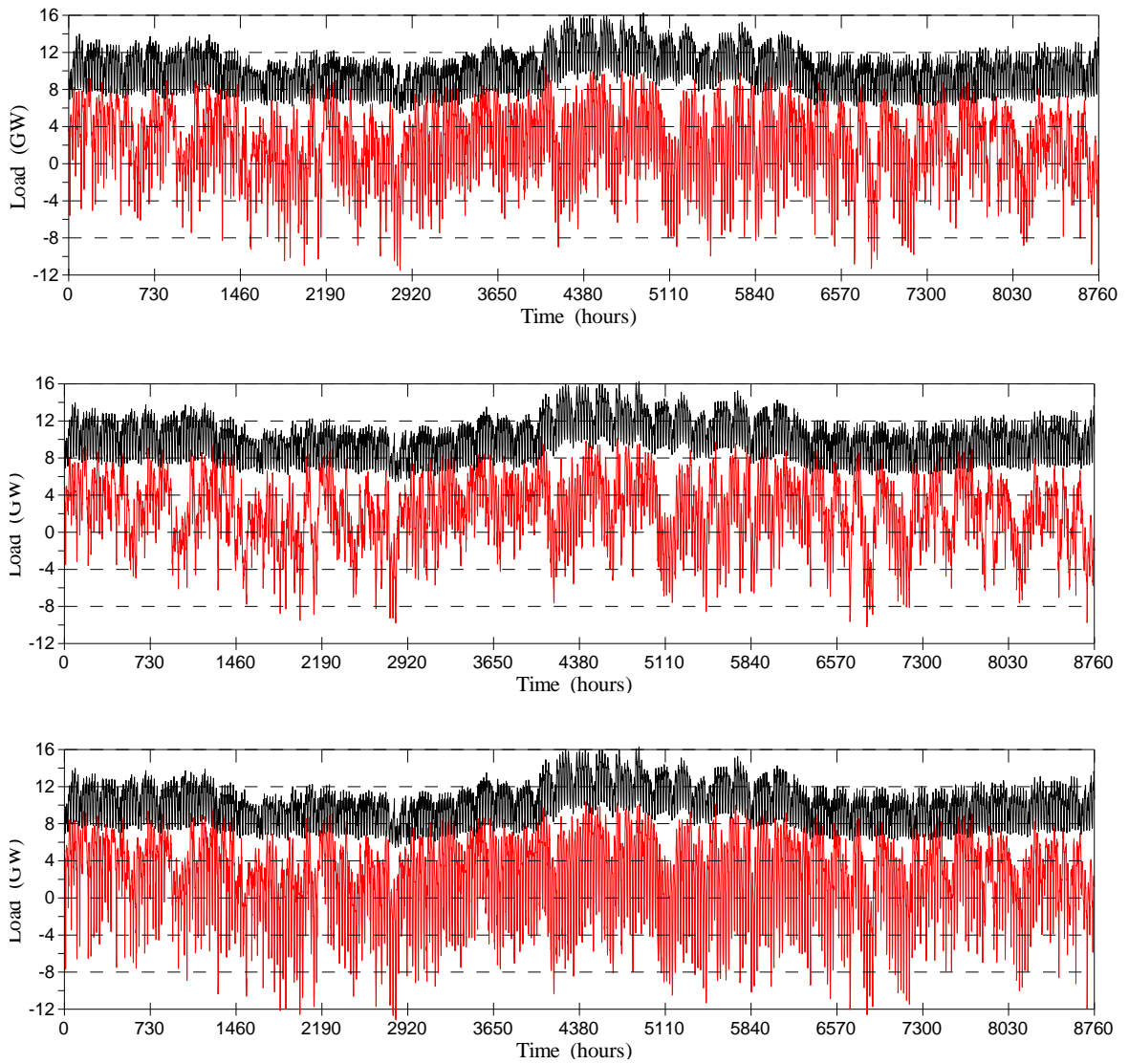
Figure 2.4. Load (black) and residual load (red) for the 80% RES share (2040-MEAP scenario), and cases A, B and C (from top to bottom).
