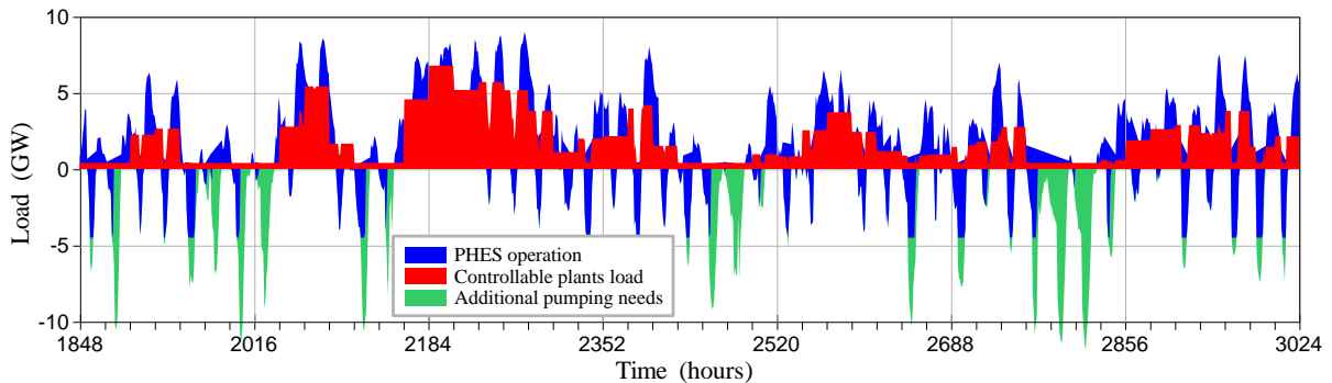
Figure 5. PHES and Controllable plants load variation for 80% scenario – case A.
