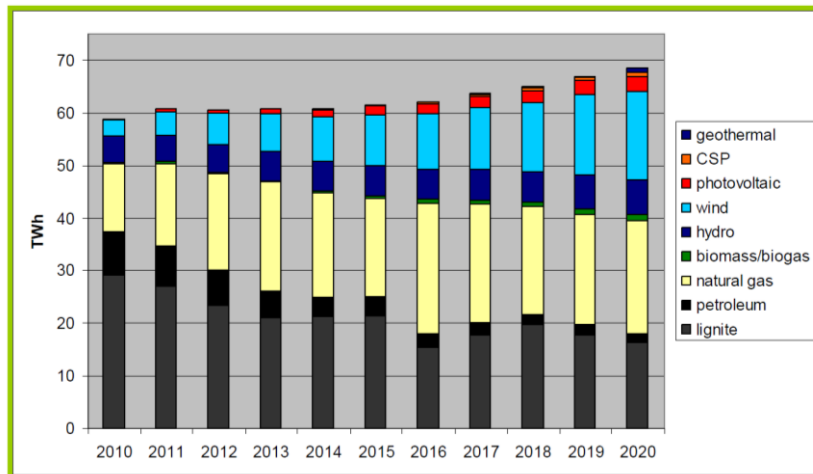
Figure 1.8. Estimated electricity generation from different technologies/fuels (National RES action plan, 2010).
