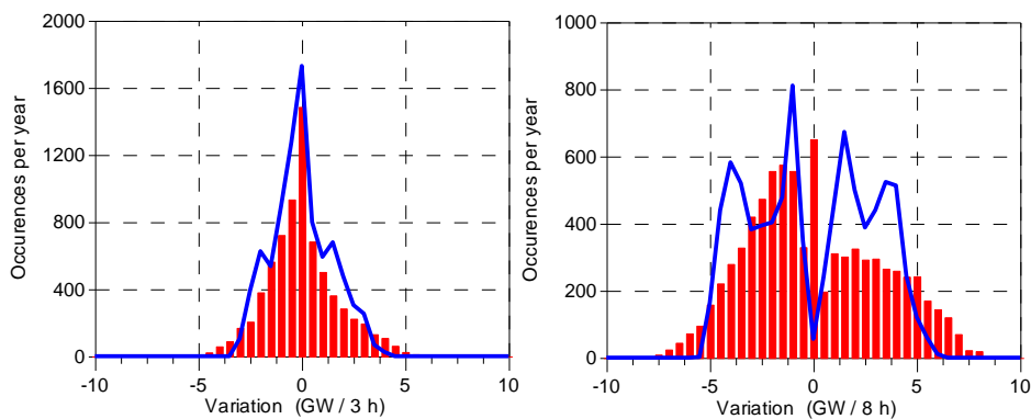
Figure 2.7. Variation of the system Load (lines) and Controllable Plants Load (bars) for the 80% scenario – Case B.
