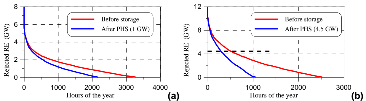
Figure 4. Duration curves of RES rejected production. a) 2020 scenario – case B, and b) 80% RES scenario – case B.
