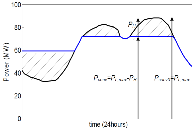
Figure 3. Indicative effects of PHES units operation on the system RL curve.
