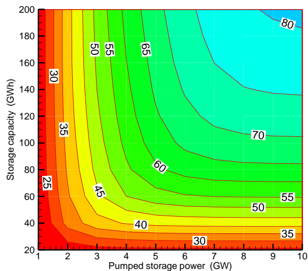
Figure 3.28. Effect of installed pumped storage power and capacity on the RES rejections exploitation degree for higher RES feed-in limit – case C.
