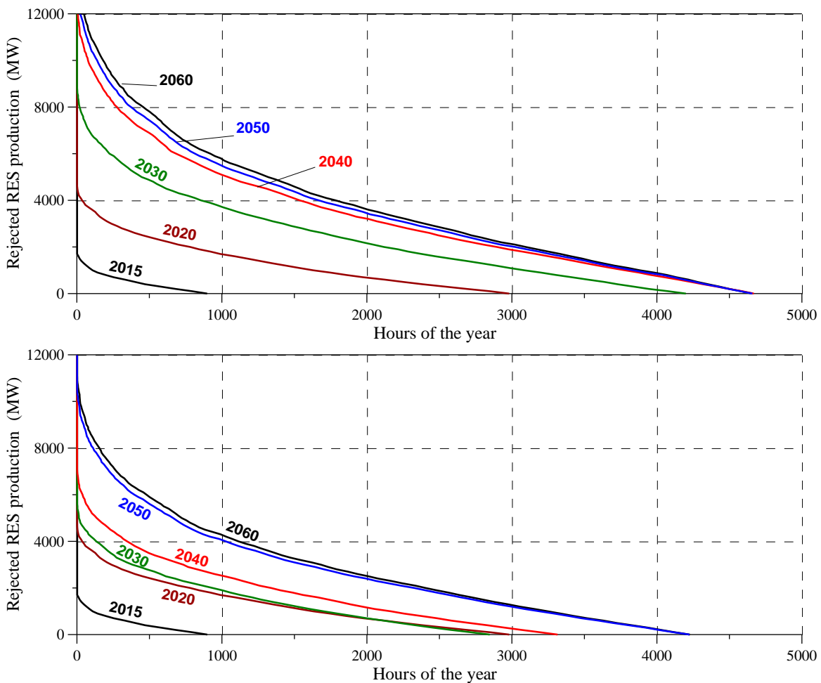
Figure 3.29. Duration curves of intermittent RES production rejections, by the energy development scenario MEAP (upper) and EP (lower), up to 2060.
