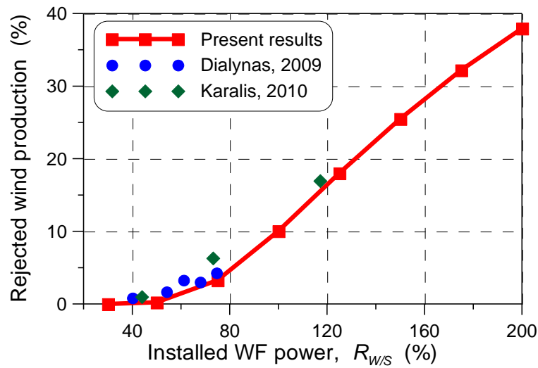
Figure A3. Annual wind energy rejection as function of the installed wind power.
