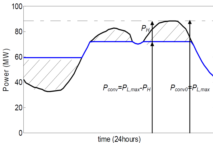
Figure A6. Indicative sketch of PHEs units operation in the electric power system.
