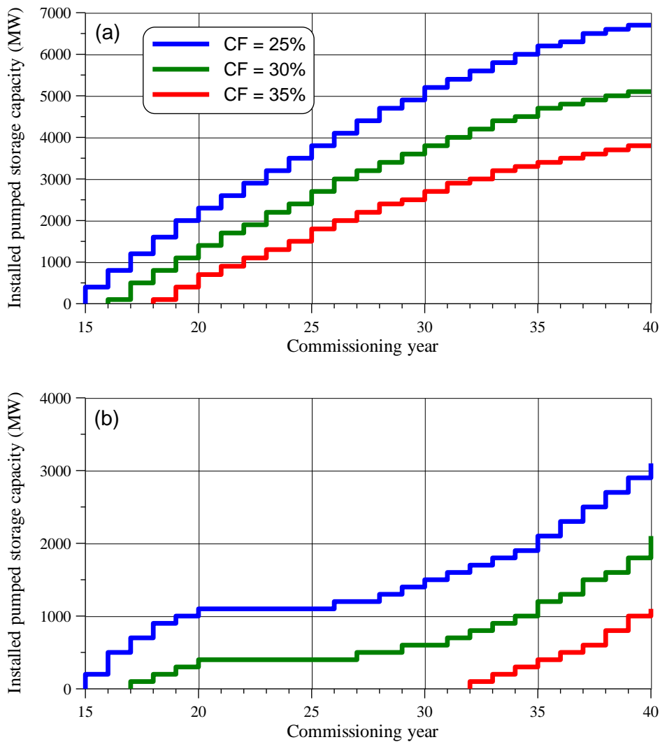
Figure 3.31. Sizing of PHES development up to 2040: a) Scenario MEAP; b) Scenario EP.
