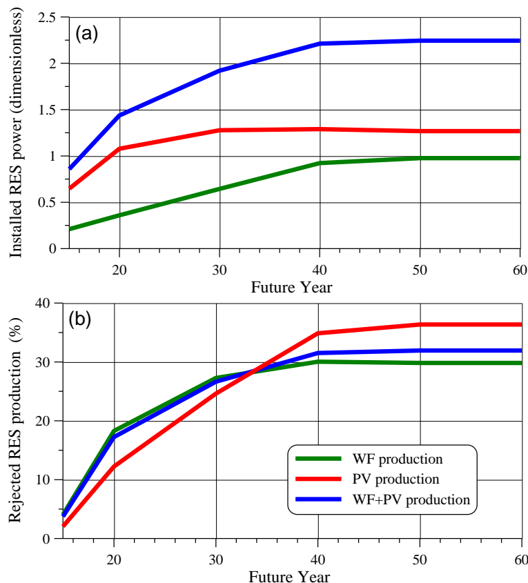
Figure A2. Intermittent RES development by scenario MEAP: a) Dimensionless installed power ( R -variables); b) Annual RES energy rejections.
