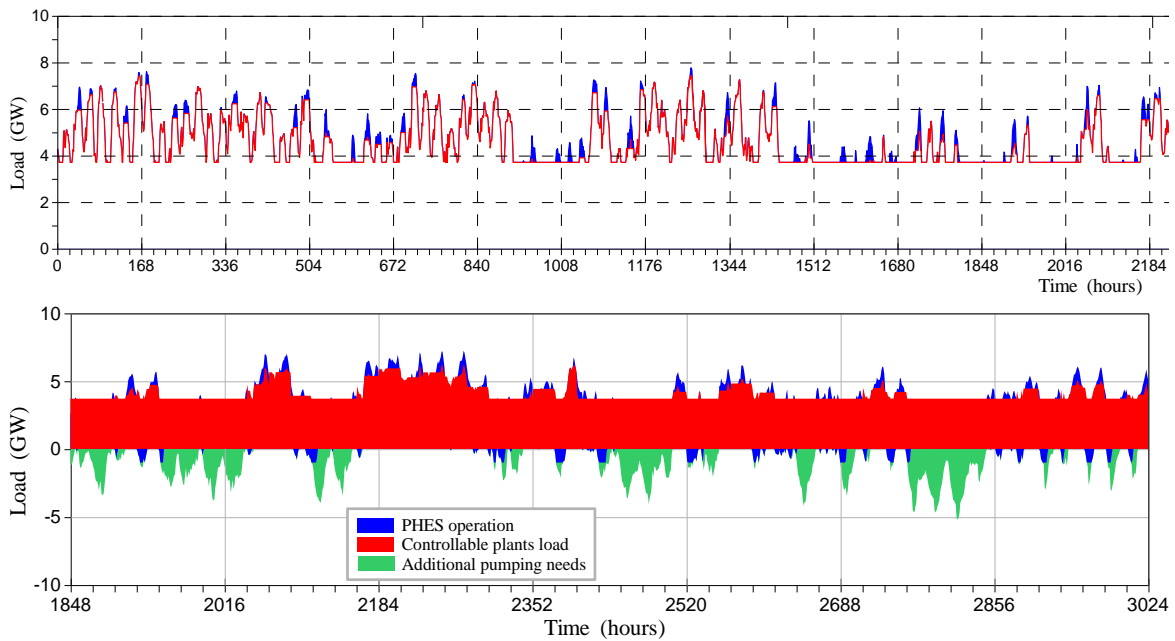
Figure 3.2. Detailed views of CPL variation and PHES performance for 40% scenario – case A.
