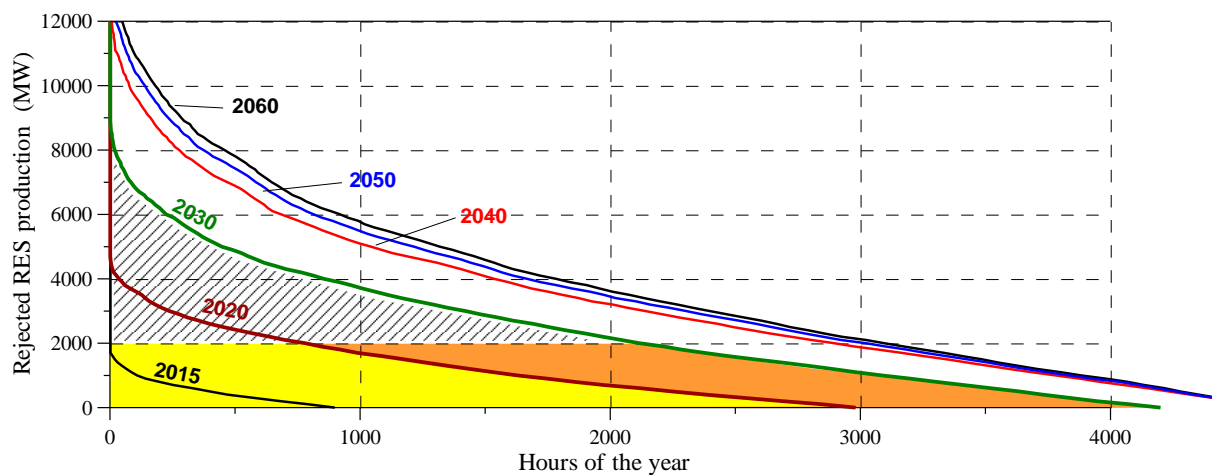
Figure 3.30. Example of rejected energy recovery by a 2 GW pumped storage unit.
