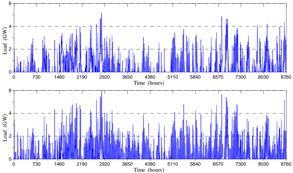
Figure 2.2. Rejected energy from intermittent RES for 40% scenario (2020), and cases A (upper) and B (lower).
