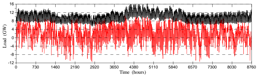
Figure 1. Load (black) and Residual Load (red) for the 80% RES scenario - case A.
