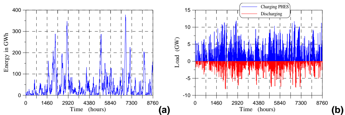
Figure 7. Charging and power level of the unlimited system, for 80% scenario – case A.
