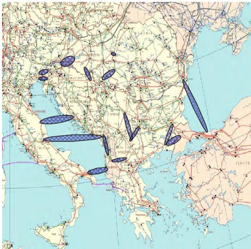
Figure 1.4. Planned new transmission lines in Balkans area (UCTE – Transmission Development Plan 2009, www.entsoe.eu ).
