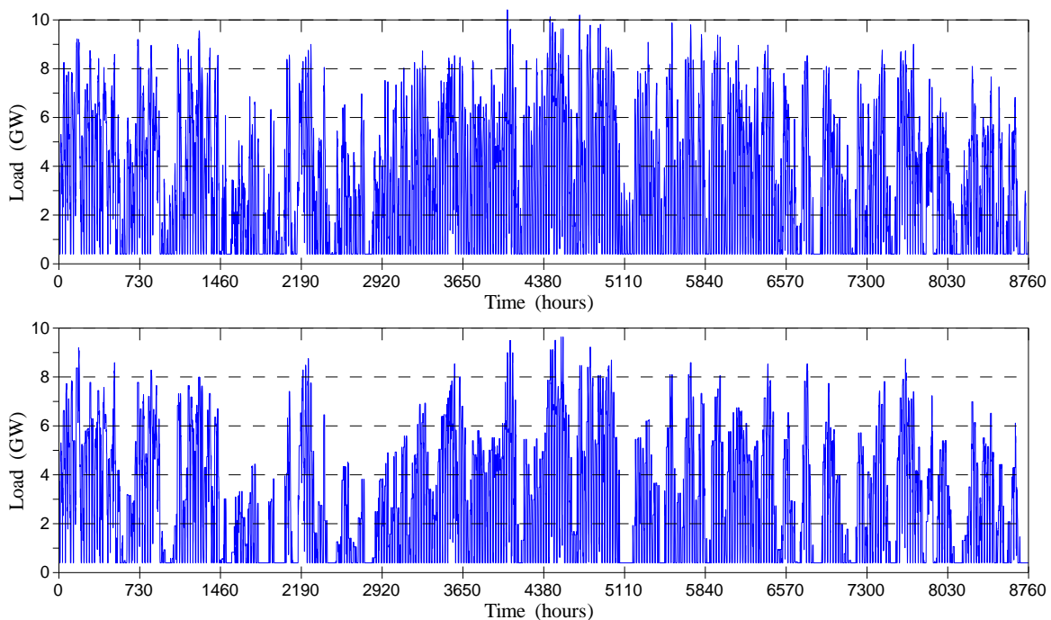
Figure 3.10. Controllable Plants Load without storage (upper) and with PHES for RES rejections (lower), for 80% scenario – case A.
