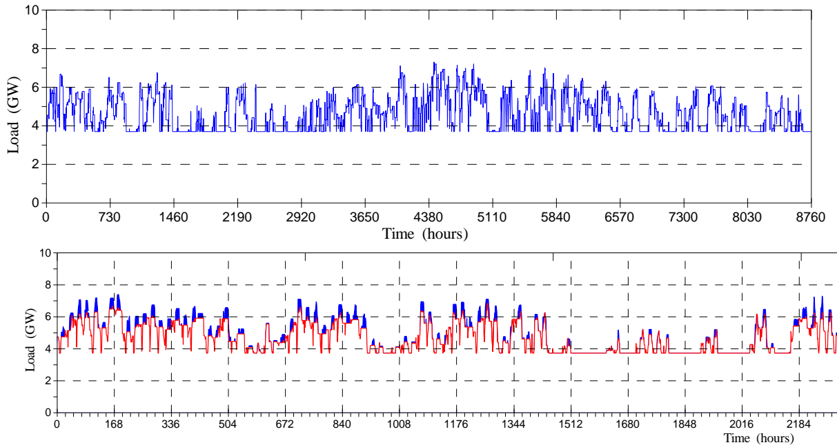
Figure 3.4. Controllable Plants Load after full PHEs exploitation (upper) and detailed view of peak shaving effect (lower) – case B.
