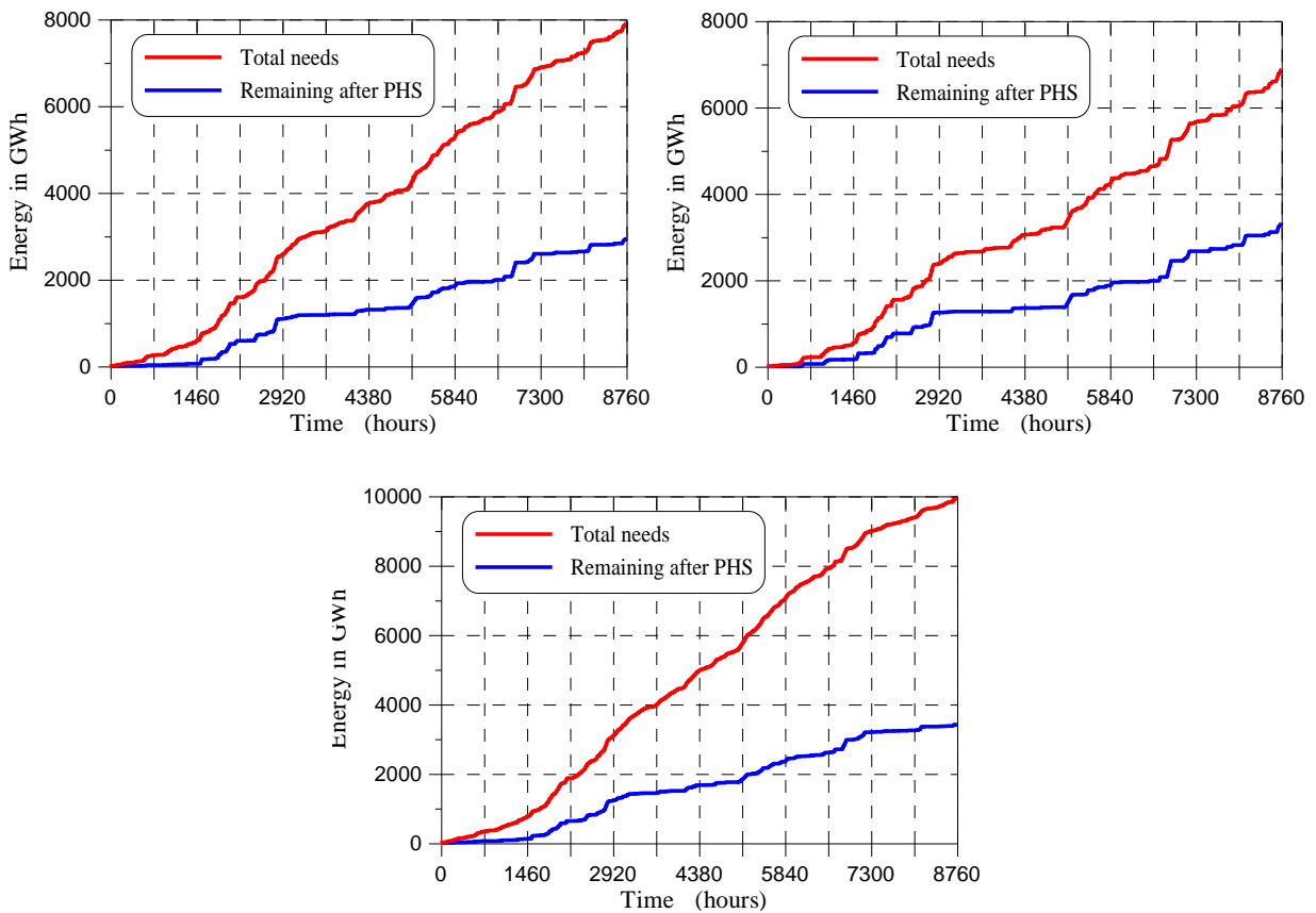
Figure 3.15. Accumulated RES energy rejections / storage needs during one year, for 80% share – cases A (upper-left), B (upper right), and C (lower).
