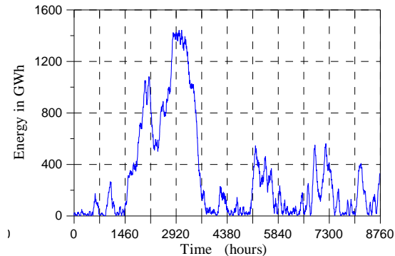
Figure 8. Storage history in case of higher technical minimum for RES penetration – case A.
