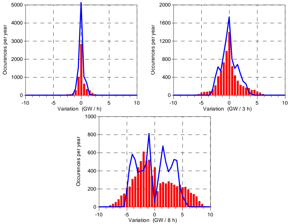
Figure 2.6. Variation of the system Load (lines) and Controllable Plants Load (bars) for the 80% scenario – case A.
