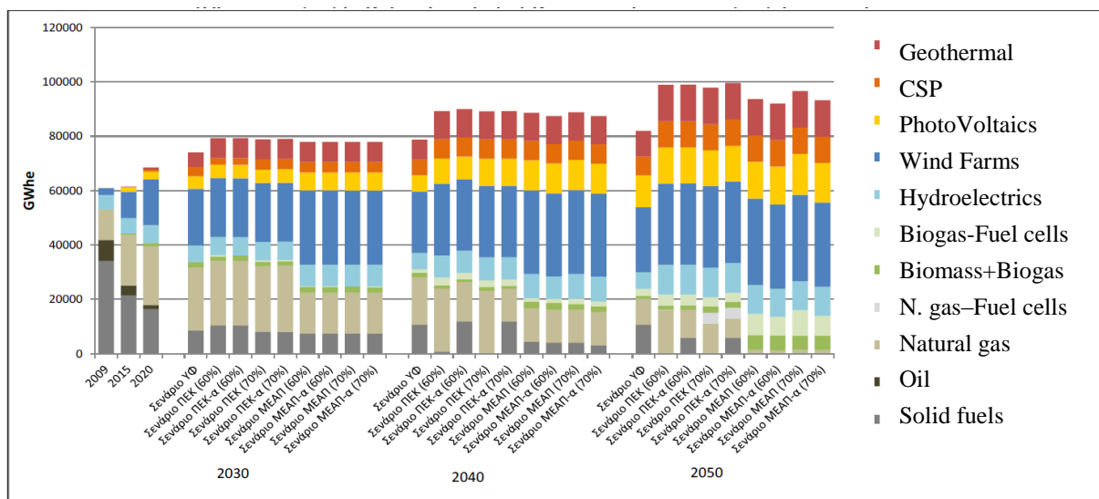
Figure 1.9. Electric energy production mix for various development scenarios [5].
