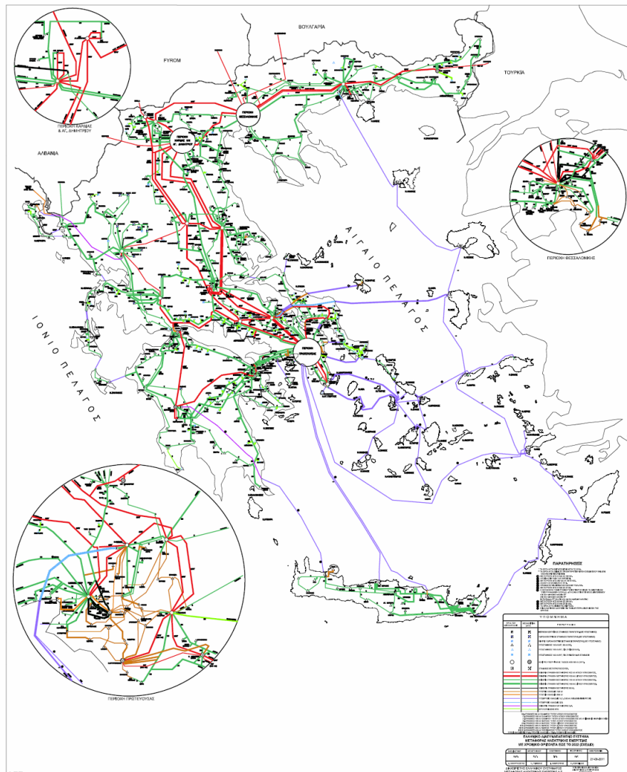
Figure 1.5. Transmission lines after interconnection of the Aegean Island ( www.admie.gr )
