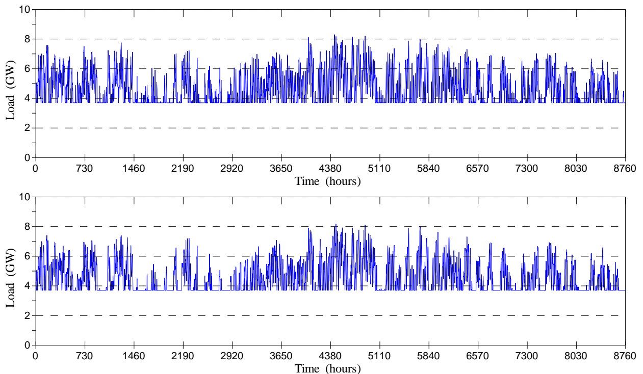
Figure 3.1. Controllable Plants Load without storage (upper), and with PHES only for RES rejections (lower), for 40% scenario – case A.
