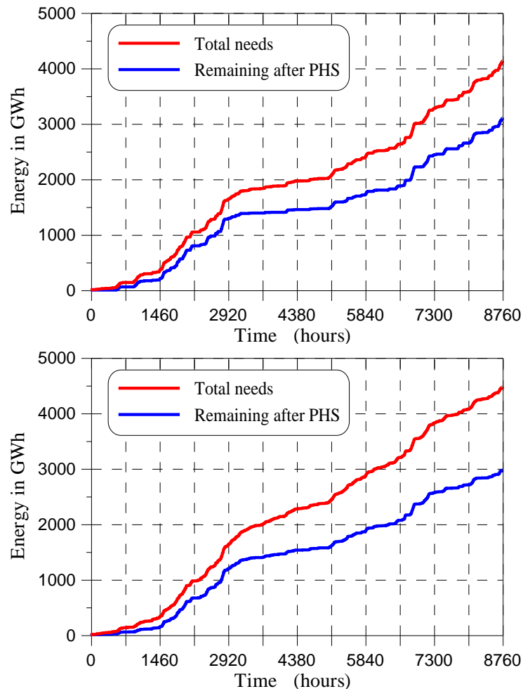
Figure 3.6. Accumulated RES energy rejections / storage needs during one year, for 40% share – cases A (upper), and B (lower).
