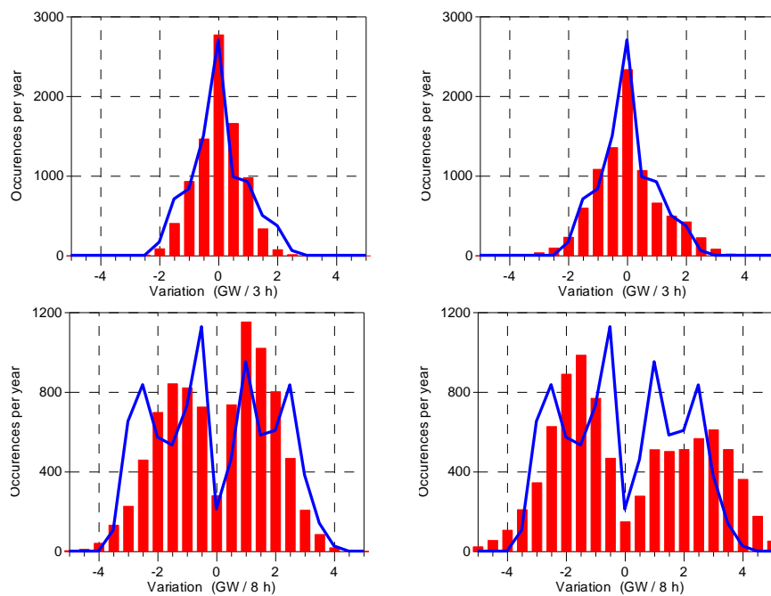
Figure 2.3 Total load variation (cont. lines) and residual load (bars) for the 40% scenario: Case A (left), and case B (right).
