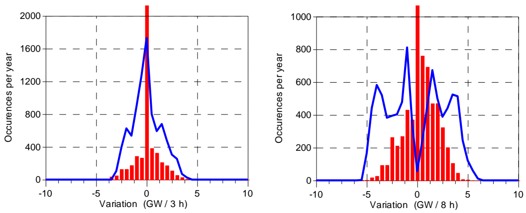
Figure 3.20. Total load variation (cont. lines) and residual load after full exploitation of the PHEC system (bars), for 80% scenario – case A.
