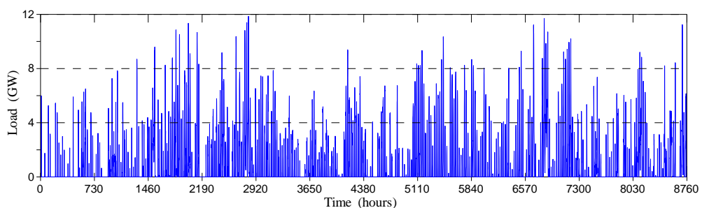
Figure 2. Rejected energy from intermittent RES for the 80% scenario - case A.
