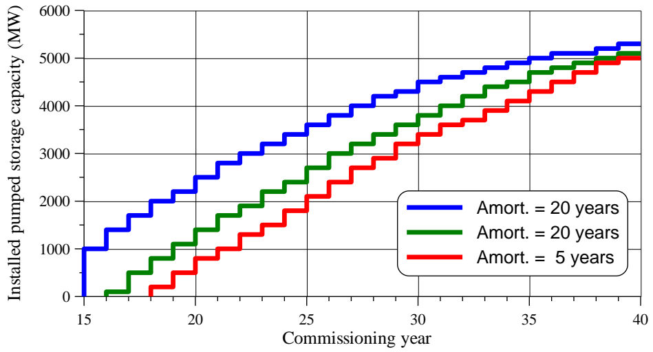
Figure 3.32. Effect of investment amortization period on the optimum PHES development.
