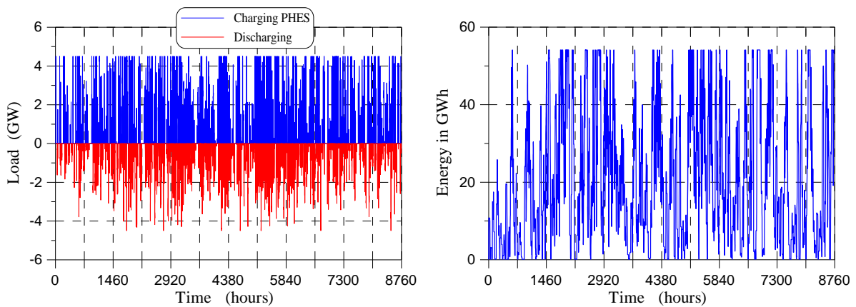
Figure 3.16. Power and charging level of PHEs system only for RES storage – case A.
